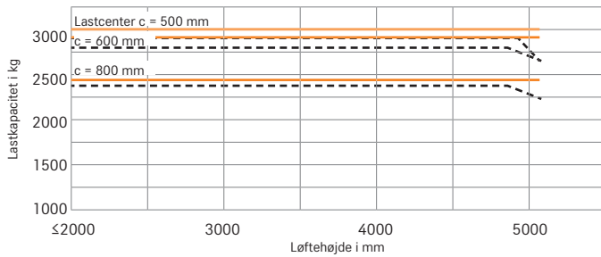
RX 60-30 dobbelt/HiLo-mast
