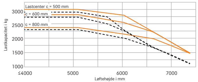
RX 60-30 Triplex-mast
