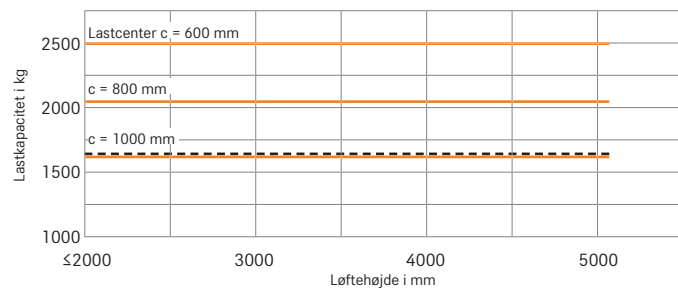
RX 60-25/600 dobbelt/HiLo-mast
