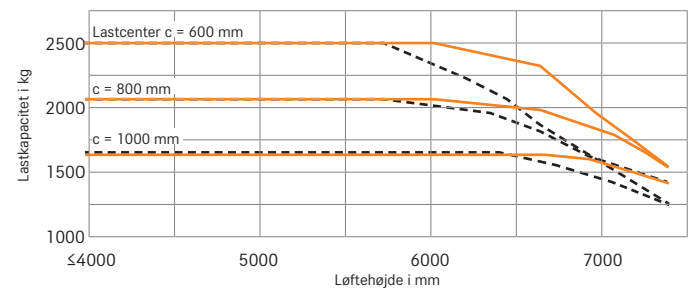
RX 60-25/600 Triplex-mast
