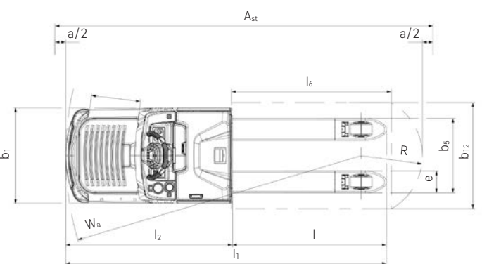
Top view backrest EXH-S
